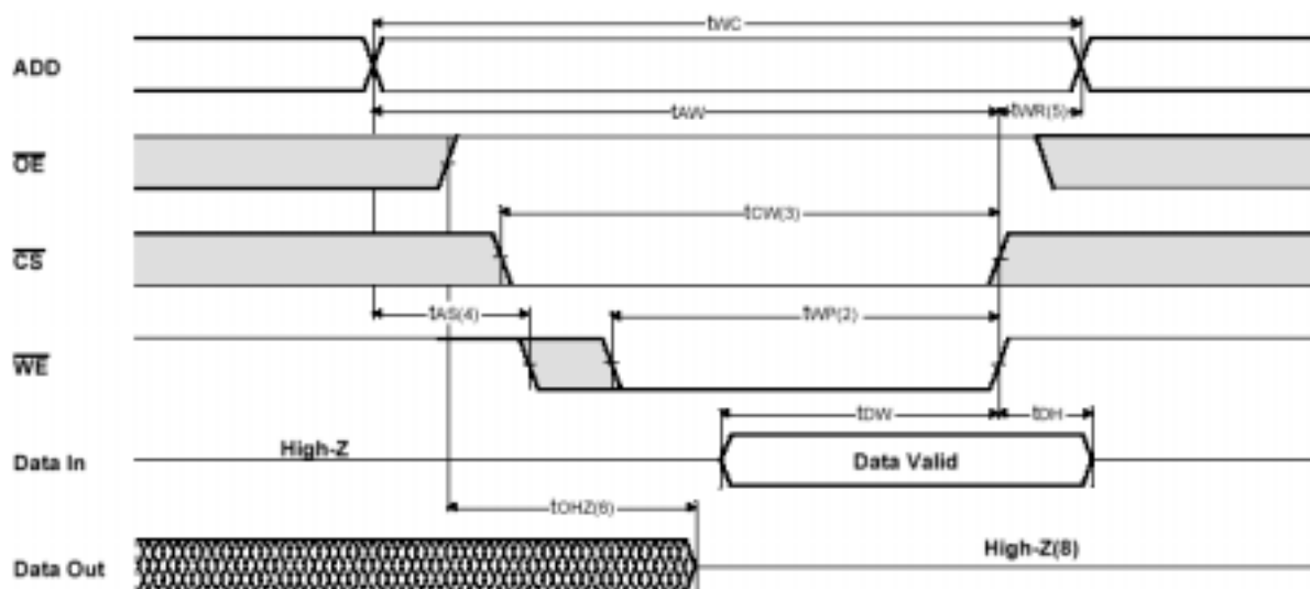
FIGURE 1. TIMING WAVEFORM OF WRITE CYCLE(1) ( \overline{\text{OE}} CLOCK)
