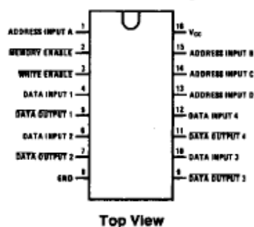
Dual-In-Line Package
