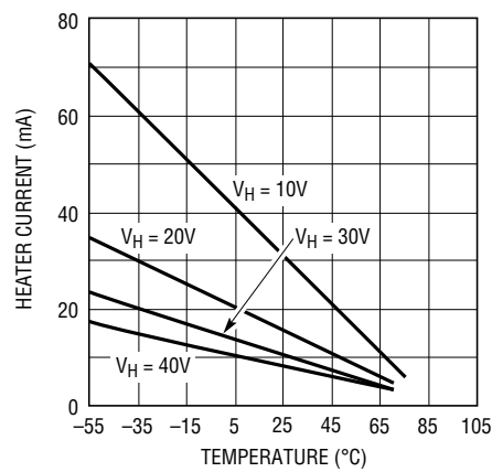
Heater Current
