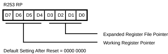
Figure 23. Register Pointer
