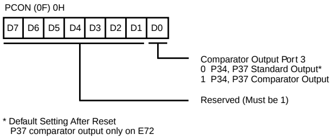
Figure 57. Port Configuration Register (PCON) ((0F) 0H: Write Only)
