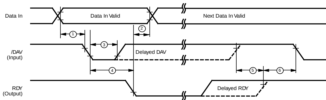
Figure 12. Input Handshake Timing
