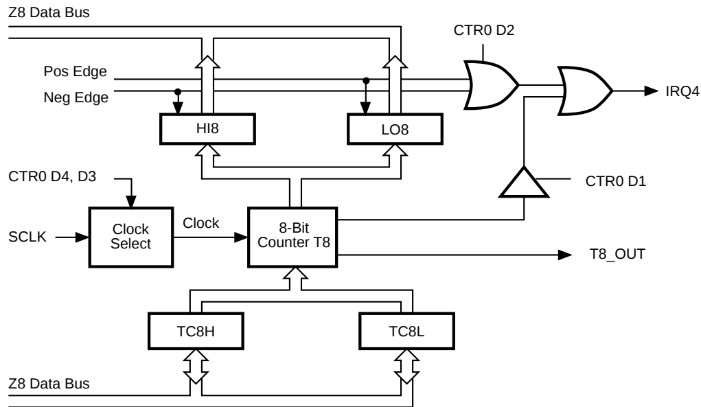
Figure 26. 8-Bit Counter/Timer Circuits
