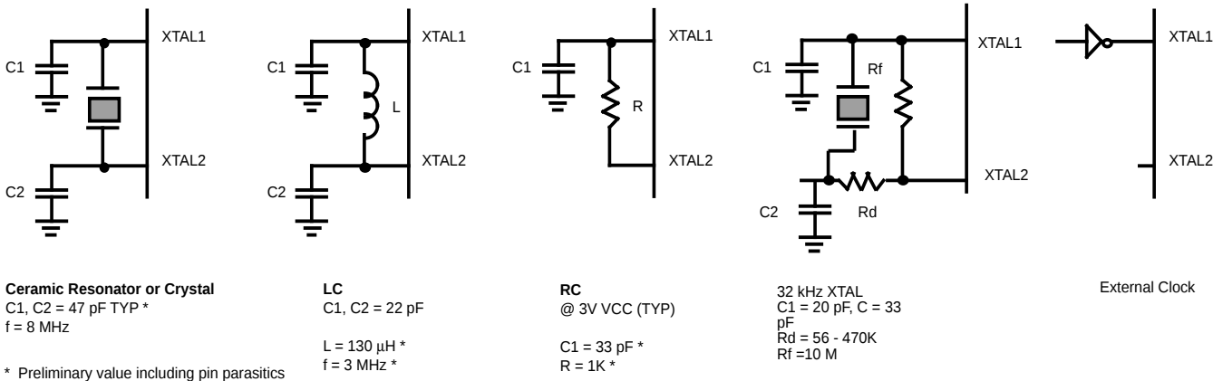
Figure 38. Oscillator Configuration
