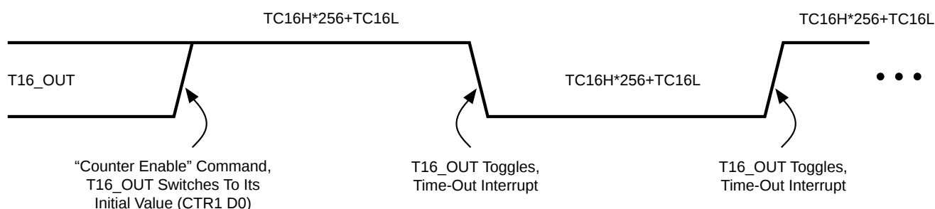
Figure 34. T16_OUT in Modulo-N Mode
