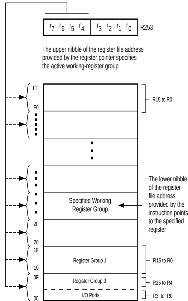
Figure 24. Register Pointer
