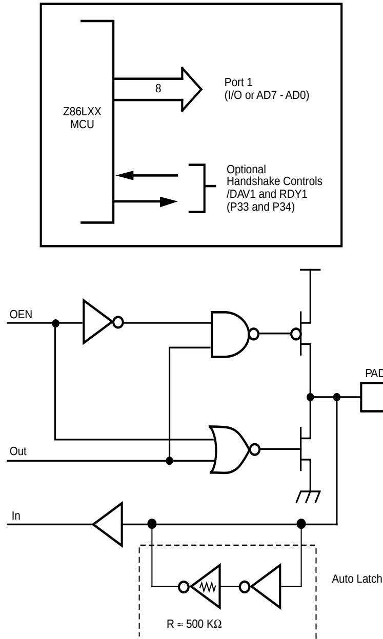
Figure 15. Port 1 Configuration
