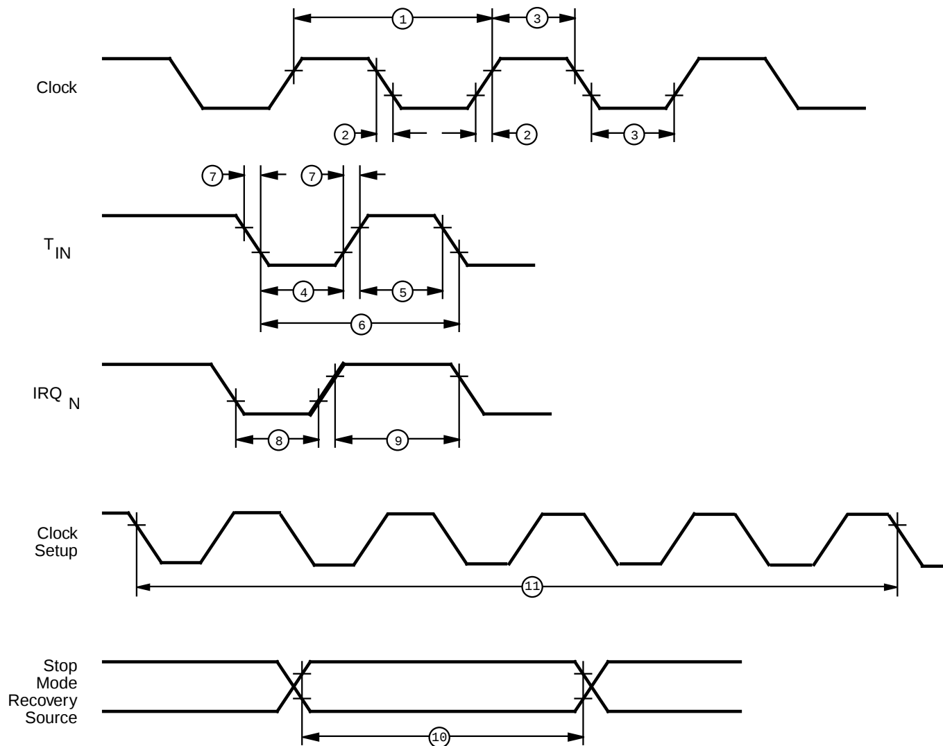
Figure 11. Additional Timing
