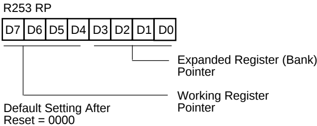
Figure 65. Register Pointer ((0) FDH: Read/Write)
