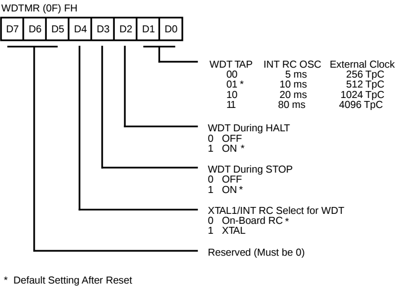
Figure 56. Watch-Dog Timer Mode Register ((F) 0FH: Write Only)
