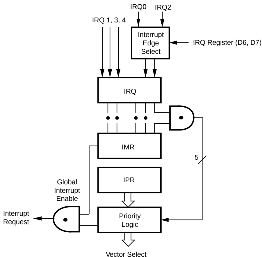
Figure 37. Interrupt Block Diagram
