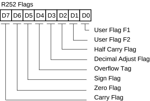
Figure 64. Flag Register ((0) FCH: Read/Write)
