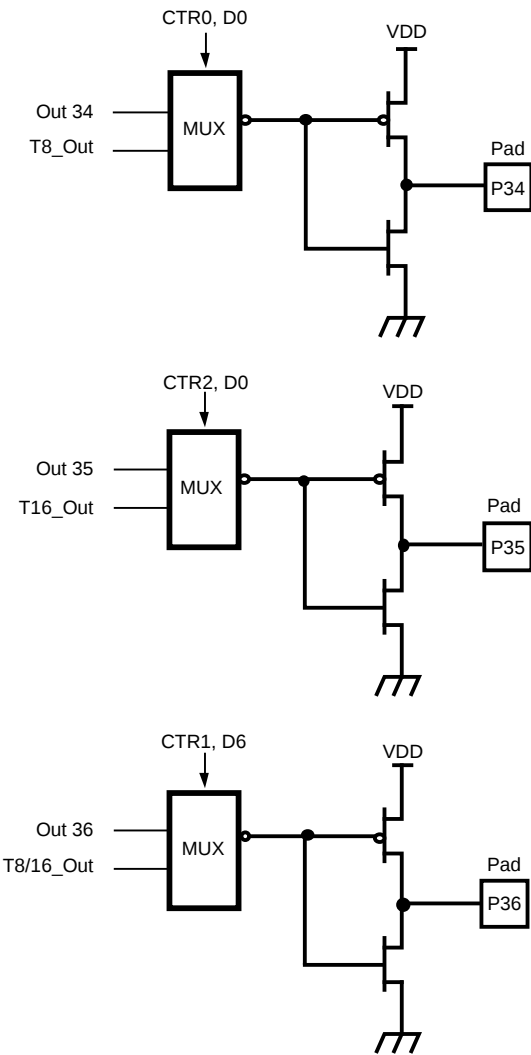
Figure 19. Port 3 Configuration
