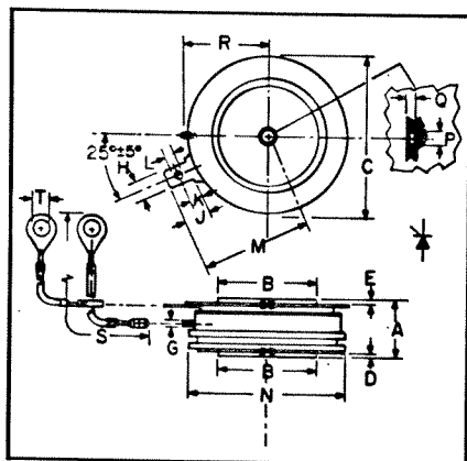
C430 Outline Drawing
