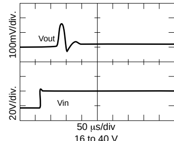
MFL2805S Step Line Response
