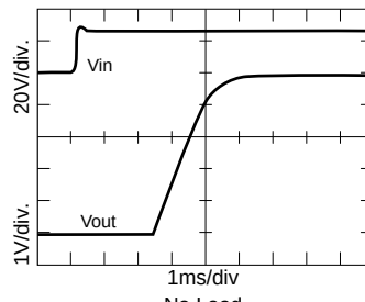
MFL2805S Turn On Response
