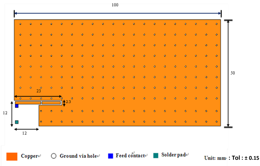
—Fig. 2 Outlook and dimension of evaluation board
