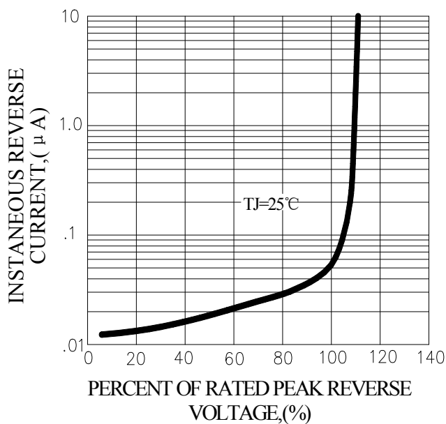
FIG.4-TYPICAL REVERSE CHARACTERISTICS
