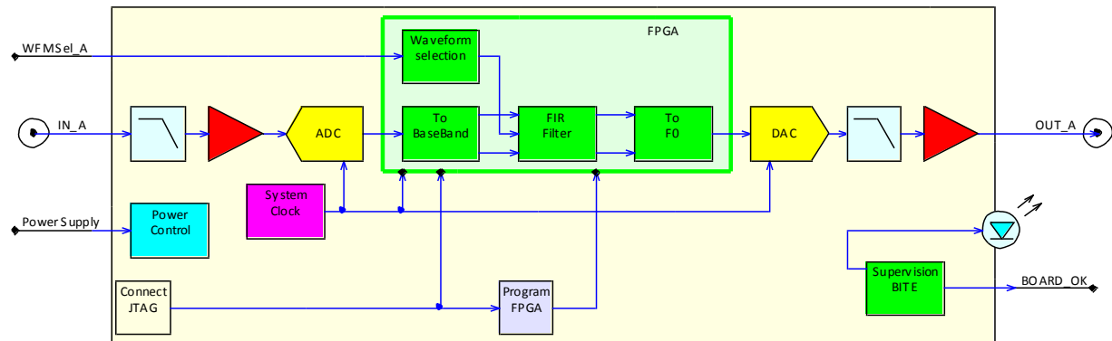
Fig. 1 : CI F04 compressor functional block diagram
