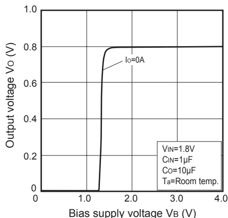
Fig.14 Output Voltage vs. Bias Supply Voltage (PQ008GN1HZPH)
