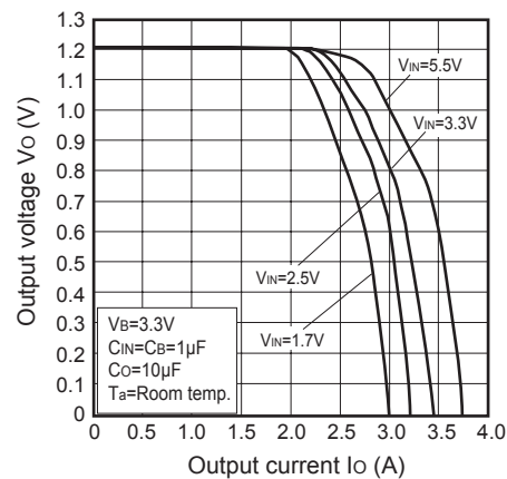
Fig.5 Overcurrent Protection Characteristics (PQ012GN1HZPH)
