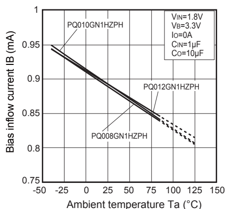
Fig.10 Bias Inflow Current vs. Ambient Temperature
