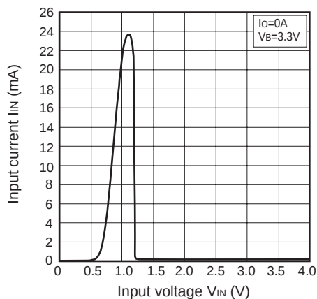
Fig.22 Input Current vs. Input Voltage (PQ012GN1HZPH)
