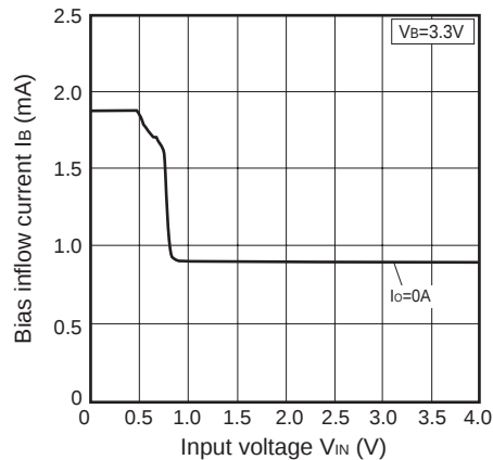
Fig.23 Bias Inflow Current vs. Input Voltage (PQ008GN1HZPH)
