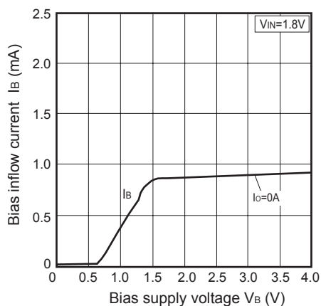
Fig.26 Bias Inflow Current vs. Bias Supply Voltage (PQ008GN1HZPH)
