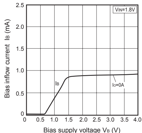
Fig.27 Bias Inflow Current vs. Bias Supply Voltage (PQ010GN1HZPH)
