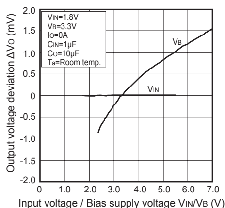
Fig.17 Output Voltage Deviation vs. Input Voltage / Bias Supply Voltage (PQ008GN1HZPH)
