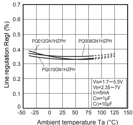
Fig.9 Line Regulation vs. Ambient Temperature
