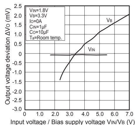
Fig.19 Output Voltage Deviation vs. Input Voltage / Bias Supply Voltage (PQ012GN1HZPH)
