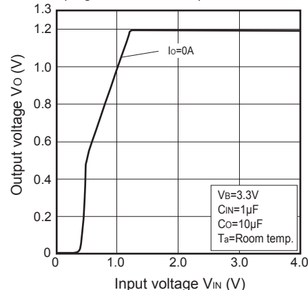
Fig.13 Output Voltage vs. Input Voltage (PQ012GN1HZPH)
