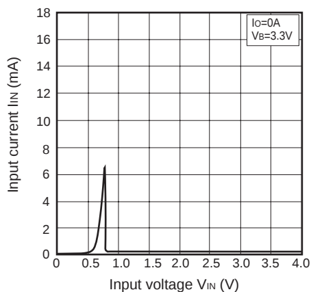
Fig.20 Input Current vs. Input Voltage (PQ008GN1HZPH)
