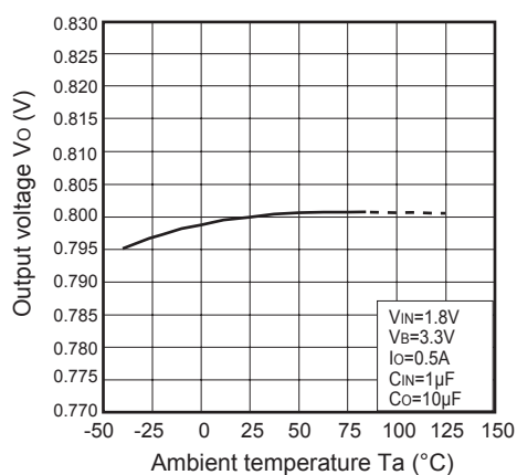
Fig.6 Output Voltage vs. Ambient Temperature (PQ008GN1HZPH)
