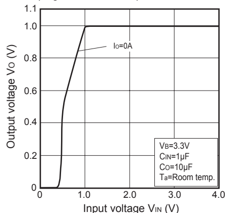
Fig.12 Output Voltage vs. Input Voltage (PQ010GN1HZPH)
