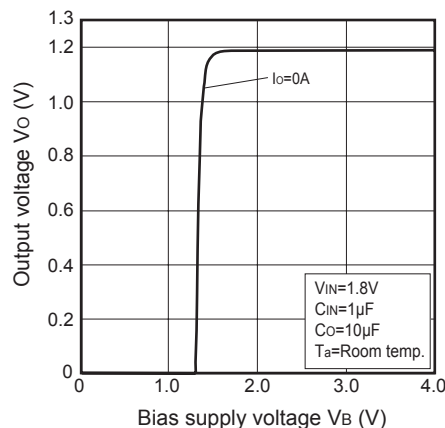
Fig.16 Output Voltage vs. Bias Supply Voltage (PQ012GN1HZPH)
