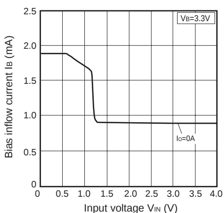
Fig.25 Bias Inflow Current vs. Input Voltage (PQ012GN1HZPH)
