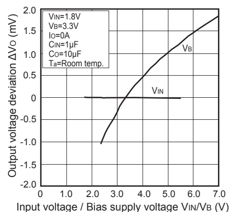
Fig.18 Output Voltage Deviation vs. Input Voltage / Bias Supply Voltage (PQ010GN1HZPH)
