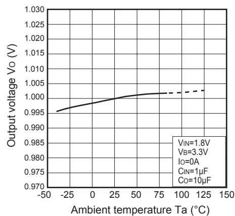
Fig.7 Output Voltage vs. Ambient Temperature (PQ010GN1HZPH)
