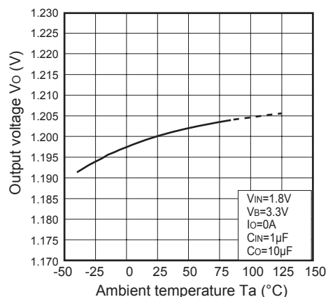
Fig.8 Output Voltage vs. Ambient Temperature (PQ012GN1HZPH)
