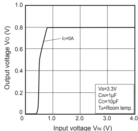
Fig.11 Output Voltage vs. Input Voltage (PQ008GN1HZPH)
