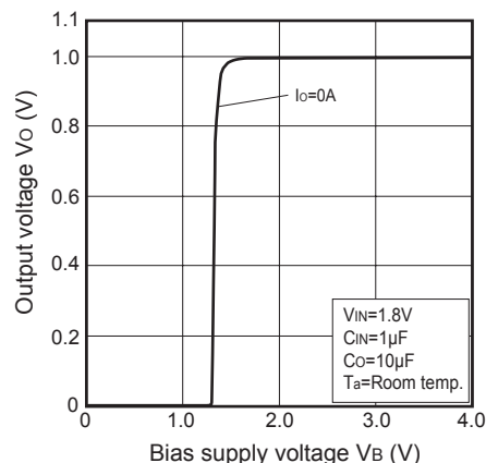
Fig.15 Output Voltage vs. Bias Supply Voltage (PQ010GN1HZPH)
