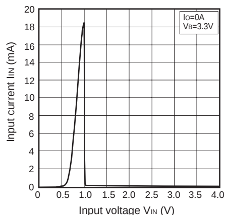
Fig.21 Input Current vs. Input Voltage (PQ010GN1HZPH)
