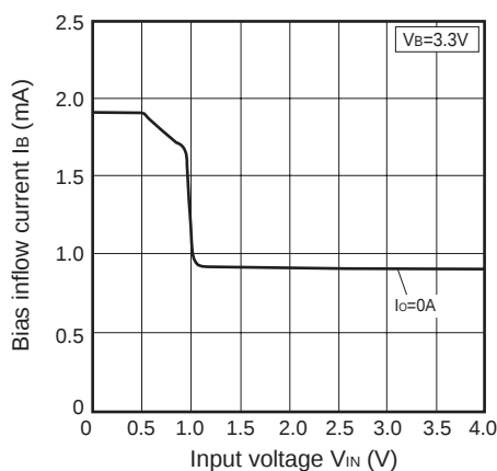
Fig.24 Bias Inflow Current vs. Input Voltage (PQ010GN1HZPH)
