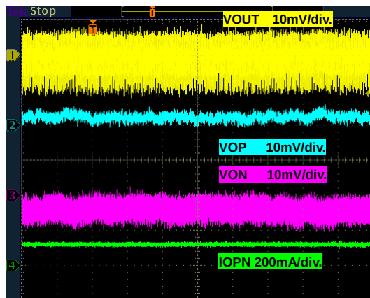
Figure 5. Steady State Heavy Load(120mA)
