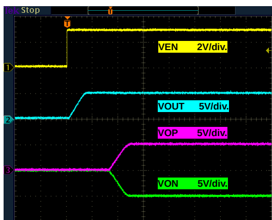
Figure 6. Power On (Simultaneous)
