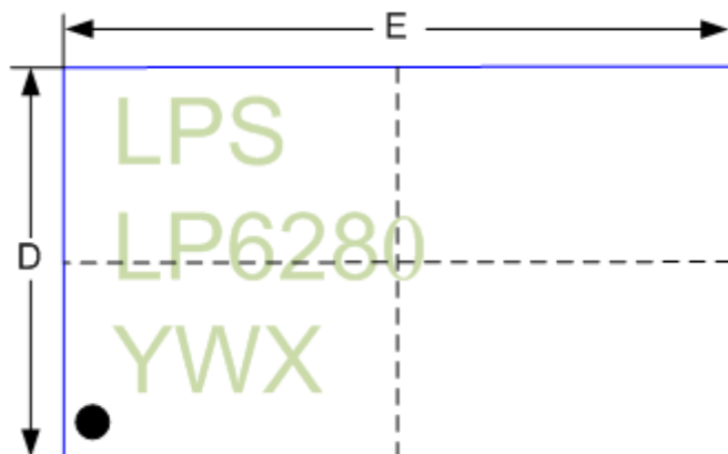
WLCSP-15-ball Package (1.4×2.3) pitch 0.4 (Unit: mm)
