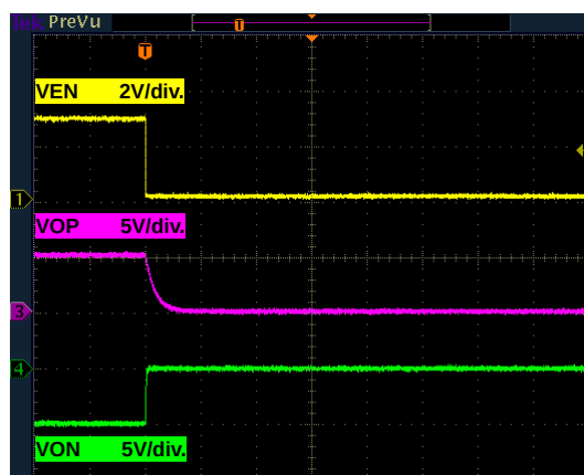
Figure 7. Power Off (Simultaneous)
