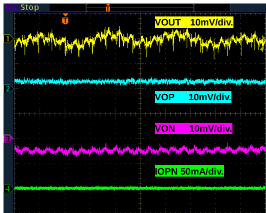
Figure 4. Steady State Light Load(0mA)
