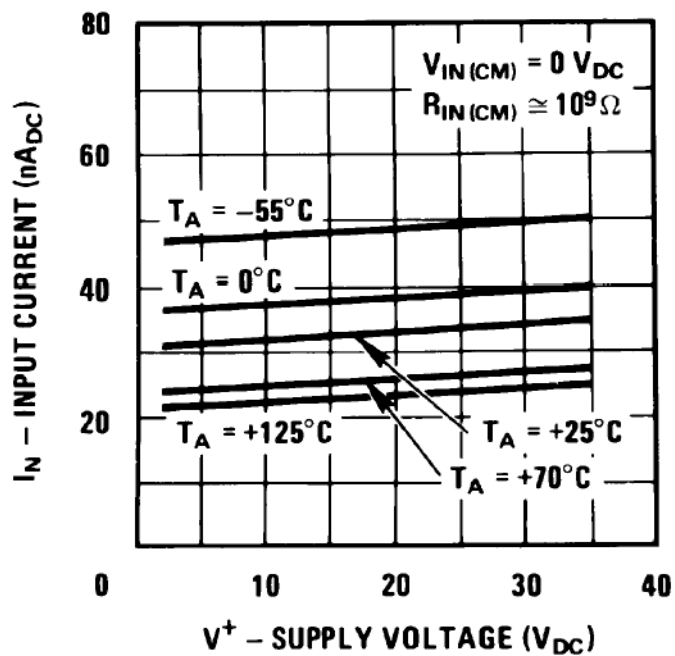
FIGURE 2. INPUT CURRENT
