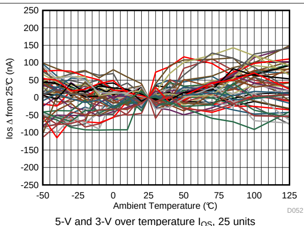
Figure 52. Input Offset Current Over Temperature
