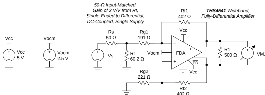
Figure 69. DC-Coupled Gain of 2 with R_f = 402\ \Omega and a Single-Ended to Differential Matched Input 50- \Omega Impedance
