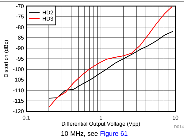
Figure 14. Harmonic Distortion vs Output Swing
