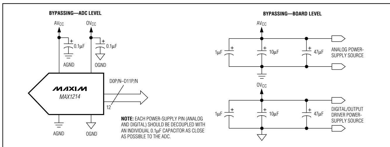
Figure 10. Grounding, Bypassing, and Decoupling Recommendations for the MAX1214
