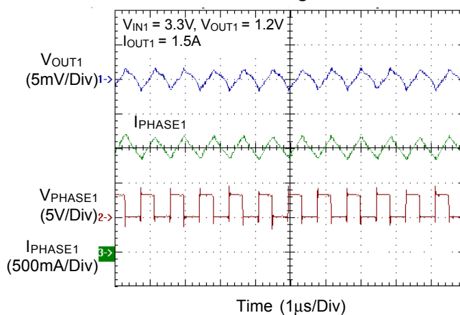
Buck Switching Waveforms
