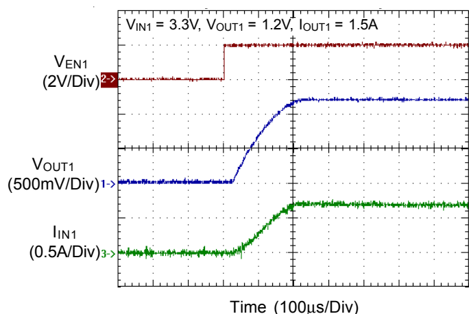
Buck Power On from EN
