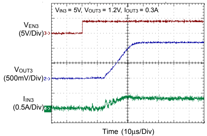
LDO2 Power On from EN3
