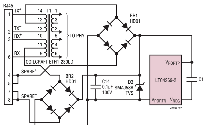
Figure 7. PD Front End with Isolation Transformer, Diode Bridges, Capacitors and a Transient Voltage Suppressor (TVS)
