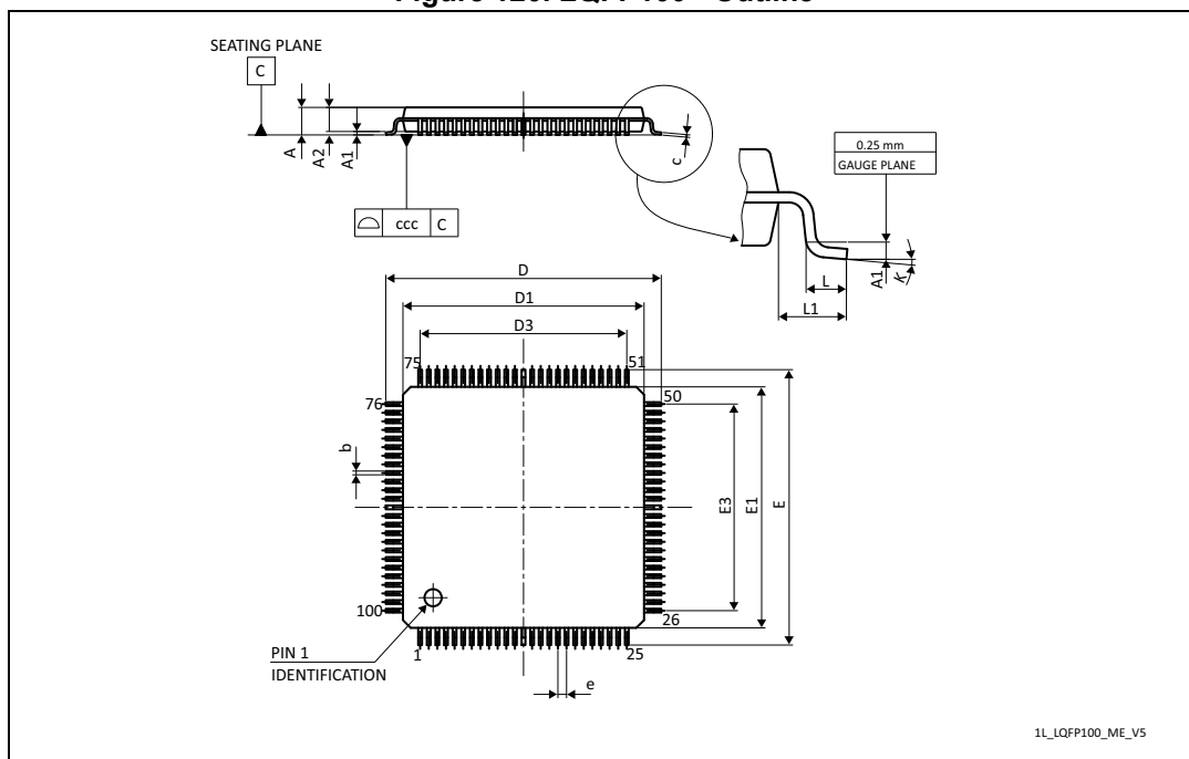
Figure 120. LQFP100 - Outline
