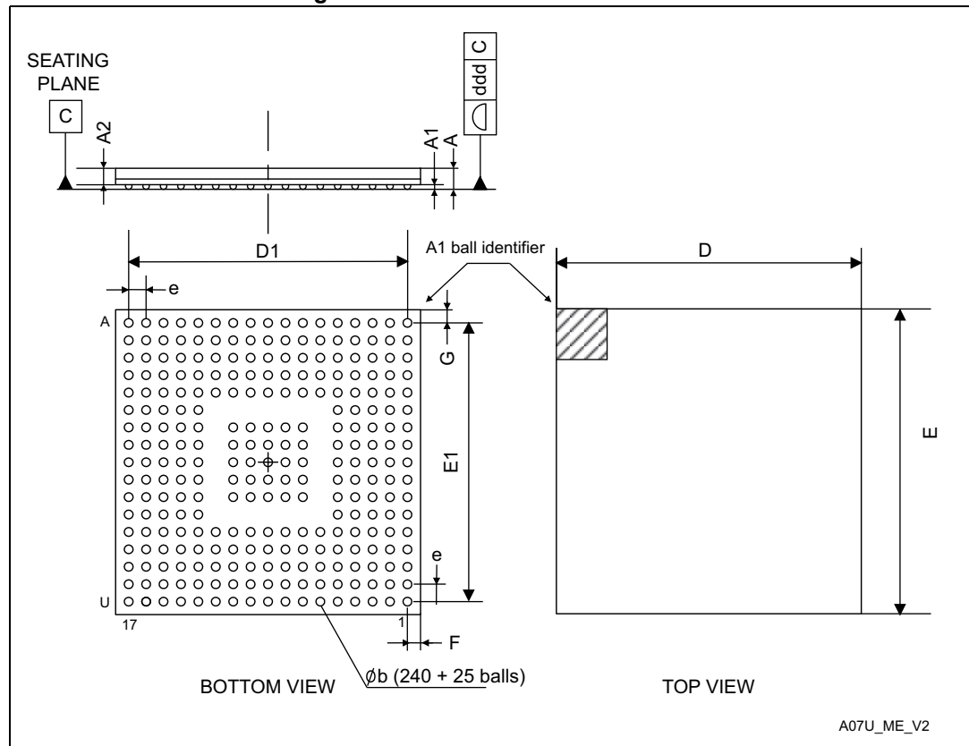
Figure 141. TFBGA240+25 - Outline
