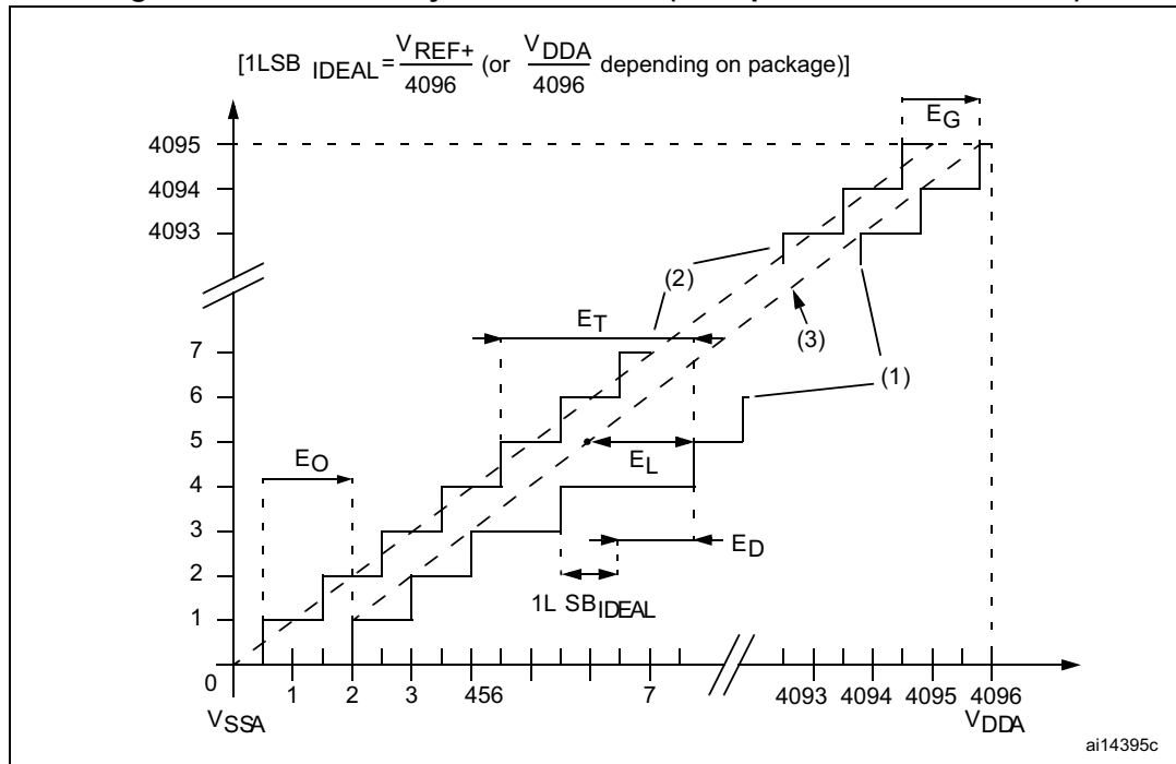
Figure 92. ADC accuracy characteristics (example for 12-bit resolution)
