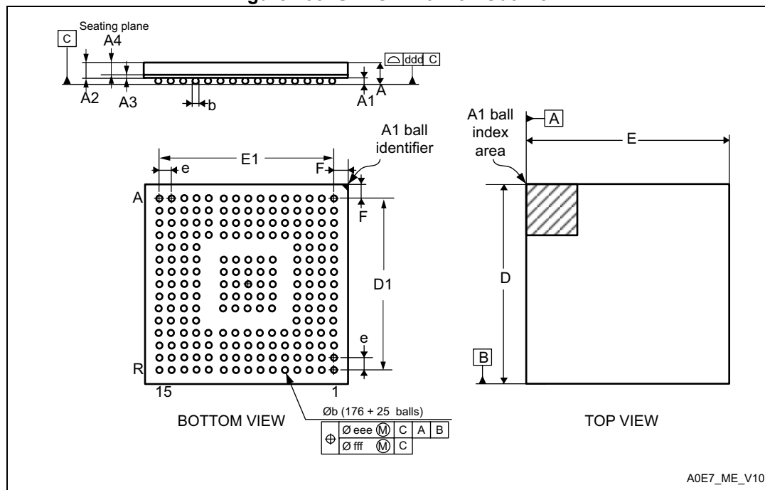
Figure 138. UFBGA176+25 - Outline
