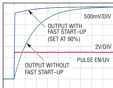
Start-Up Time with and without Fast Start-Up Circuitry for Large C_{SET}
