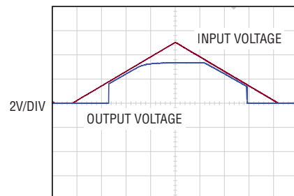
Input Supply Ramp-Up and Ramp-Down
