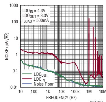
Noise Spectral Density
