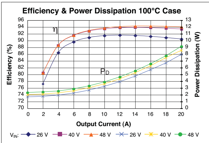
Figure 3c – Efficiency and power dissipation at 100°C (case); V_{IN}
