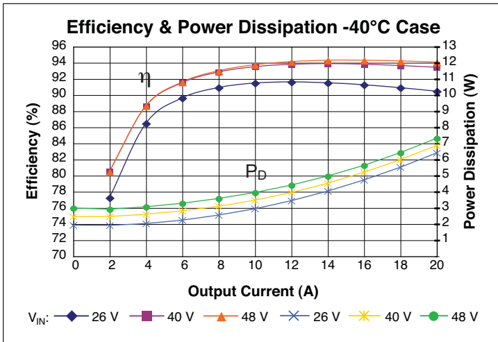
Figure 3a – Efficiency and power dissipation at -40°C (case); V_{IN}
