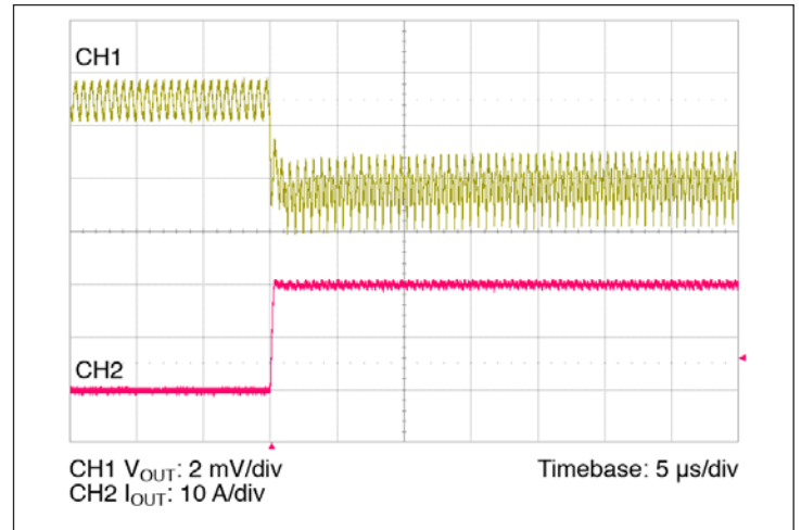
Figure 12 – 0 – 20 A transient response; C_{IN} = 100 \mu F , no external C_{OUT}
