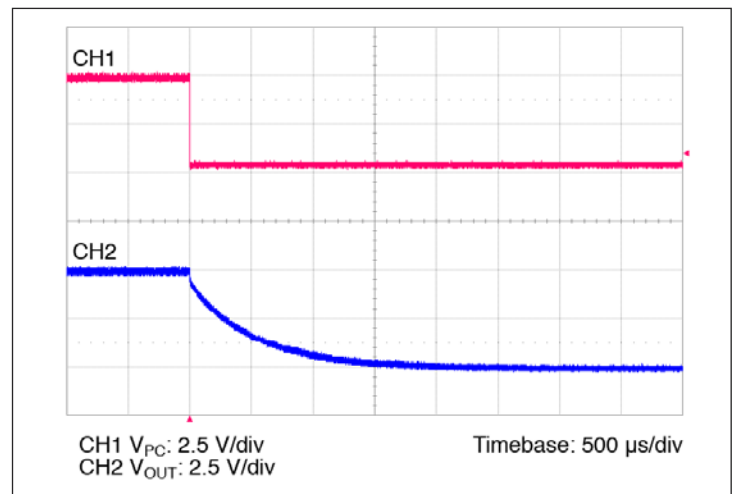
Figure 14 – PC disable waveform; R_{LOAD} = 0.25 \Omega , C_{OUT} = 1,000 \mu F
