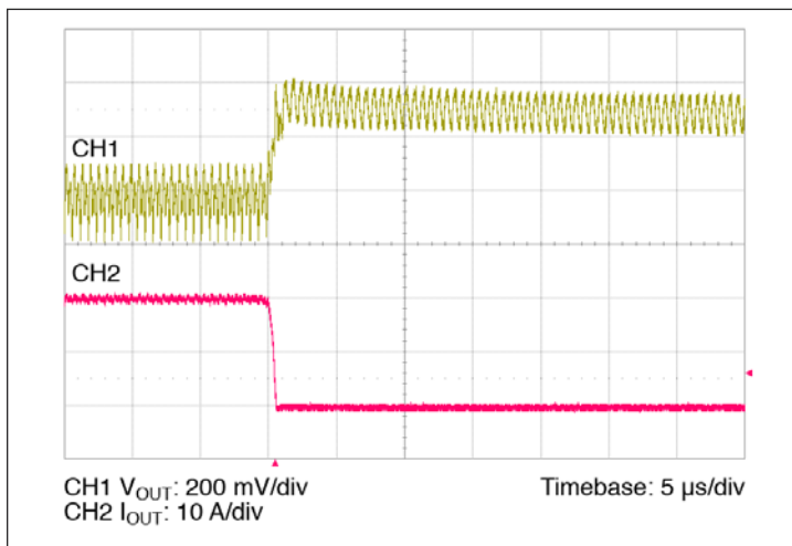
Figure 13 – 20 A – 0 A transient response; C_{IN} = 100 \mu F , no external C_{OUT}
