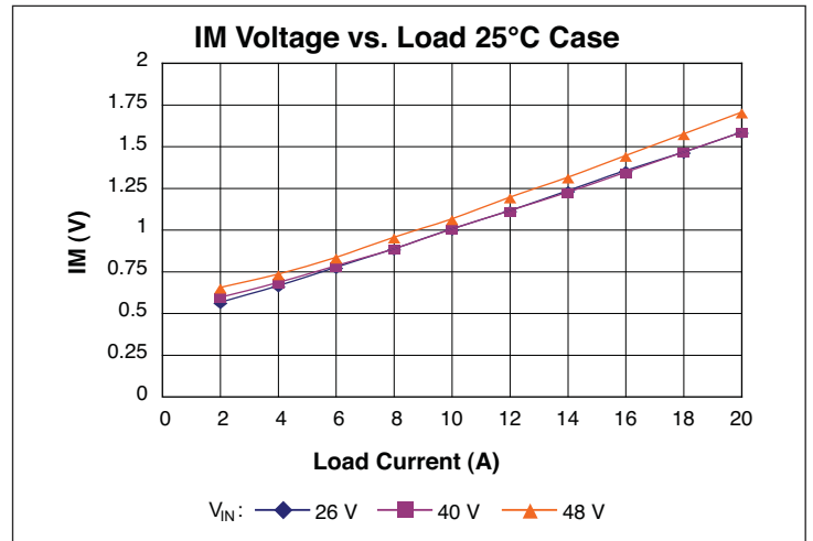
Figure 8 – IM voltage vs. load; 25°C Case
