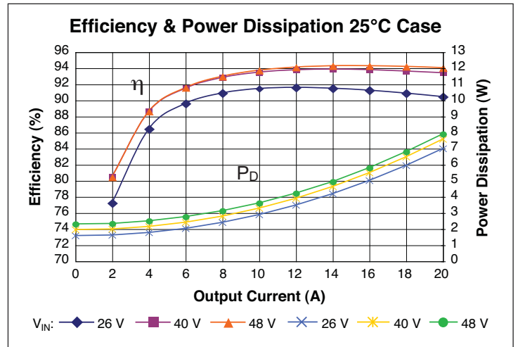
Figure 3b – Efficiency and power dissipation at 25°C (case); V_{IN}
