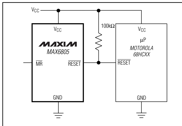
Figure 1. Interfacing to μPs with Bidirectional Reset Pins
