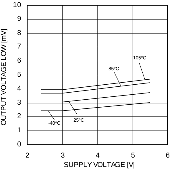
Figure 31. Maximum Output Voltage Low – Supply Voltage (RL=10kΩ)
