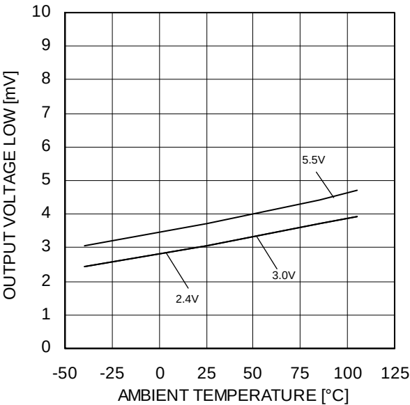
Figure 32. Maximum Output Voltage Low – Ambient Temperature (RL=10kΩ)
