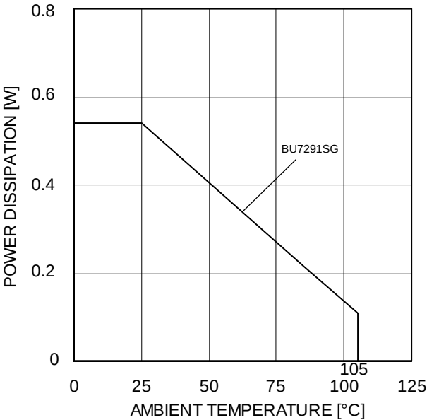
Figure 3. Derating curve
