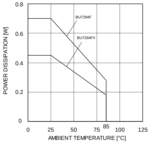
Figure 25. Derating curve
