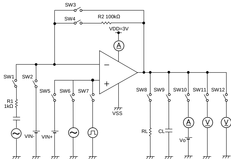
Figure 49. Test circuit 2
