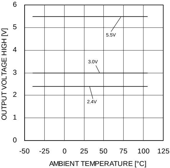
Figure 30. Maximum Output Voltage High – Ambient Temperature (RL=10kΩ)
