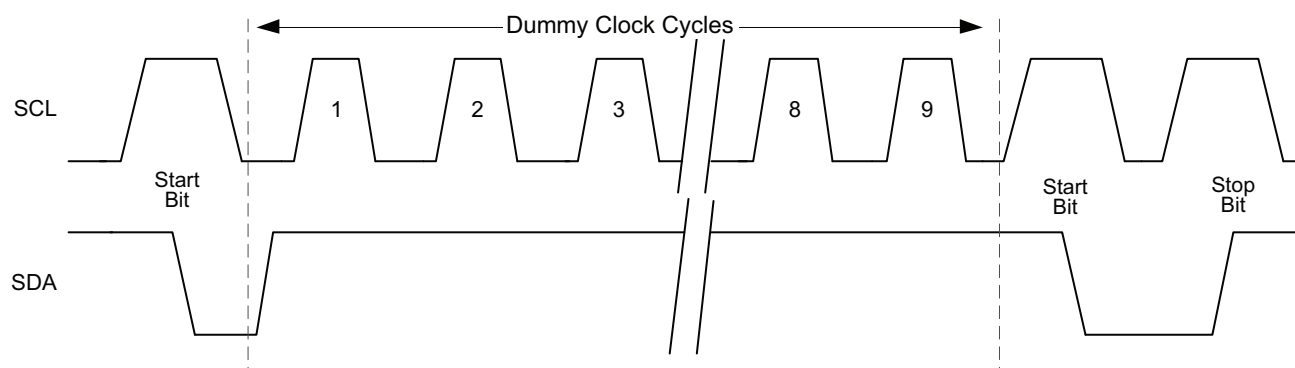
Figure 5-4. Software Reset
