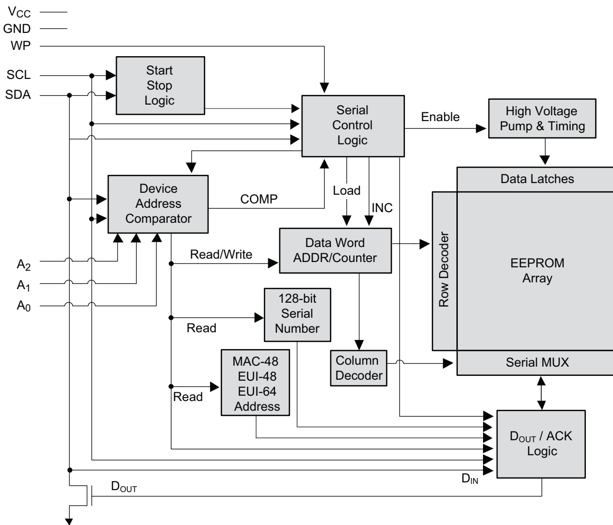
Figure 2-1. Block Diagram
