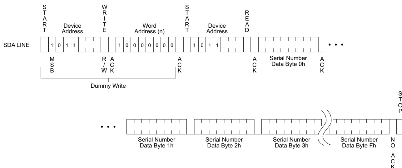
Figure 9-4. Serial Number Read
