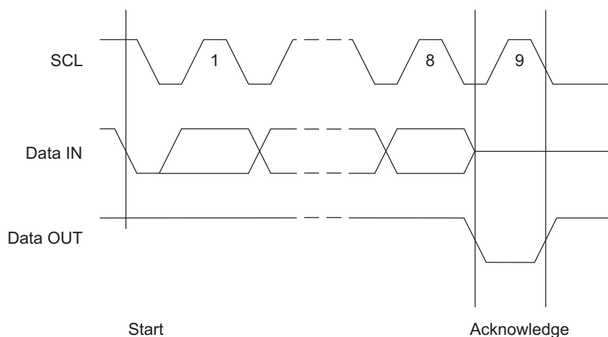
Figure 5-3. Output Acknowledge
