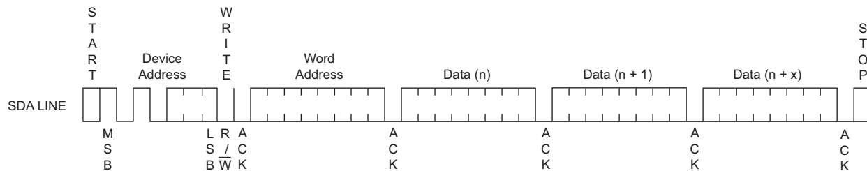
Figure 7-2. Page Write
