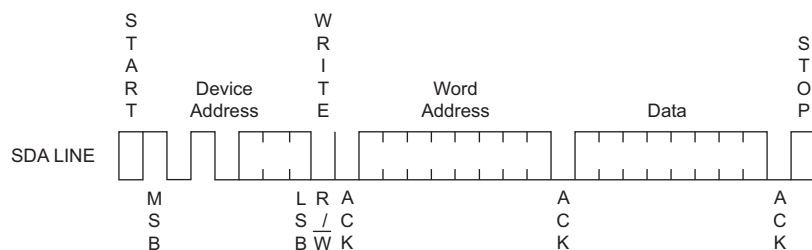
Figure 7-1. Byte Write
