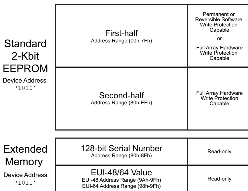
Figure 4-1. Memory Organization
