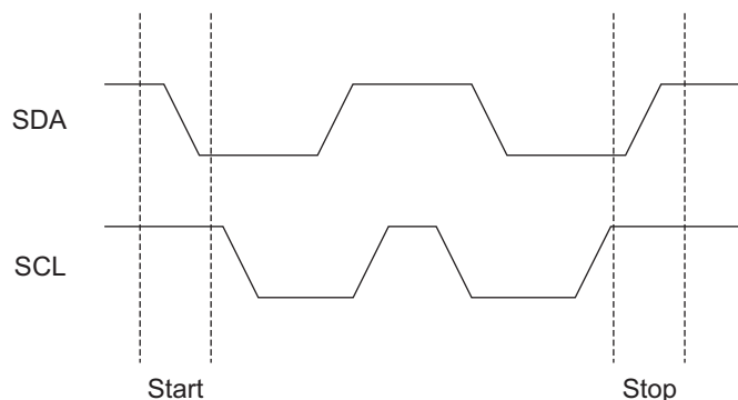
Figure 5-2. Start and Stop Condition
