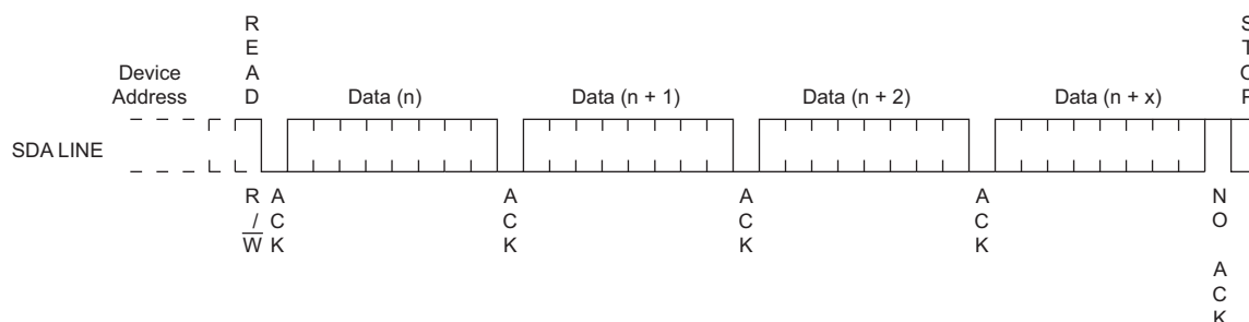
Figure 9-3. Sequential Read
