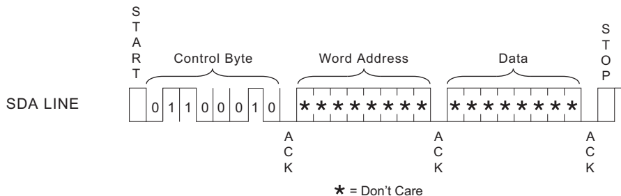
Figure 8-2. Setting Reversible Write Protect Register (RSWP)
