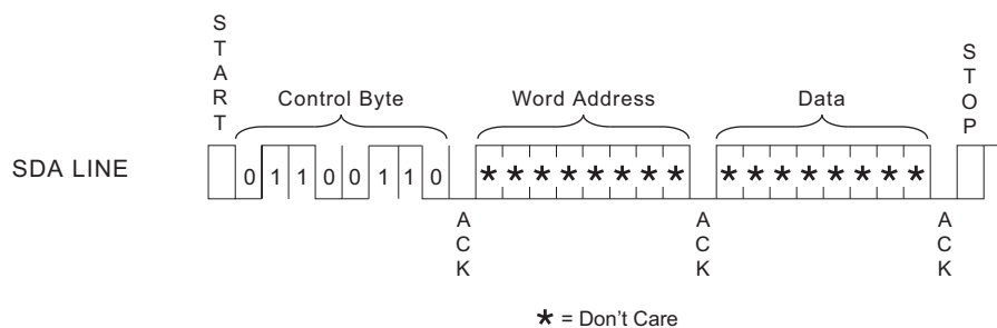
Figure 8-3. Clearing Reversible Write Protect Register (RSWP)
