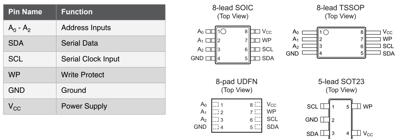
Figure 1. Pin Configurations
