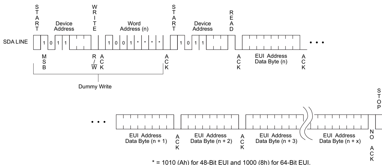
Figure 9-5. EUI Address Read
