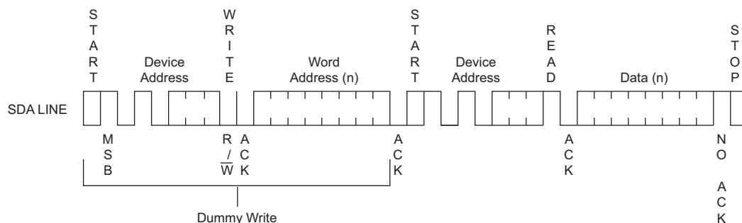
Figure 9-2. Random Read
