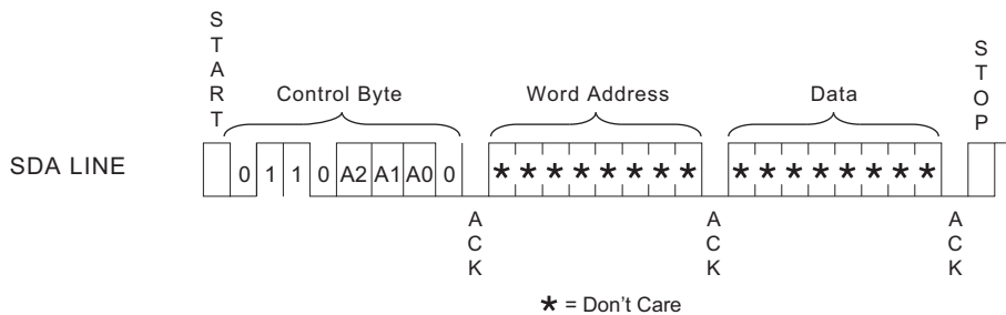
Figure 8-1. Setting Permanent Write Protect Register (PSWP)
