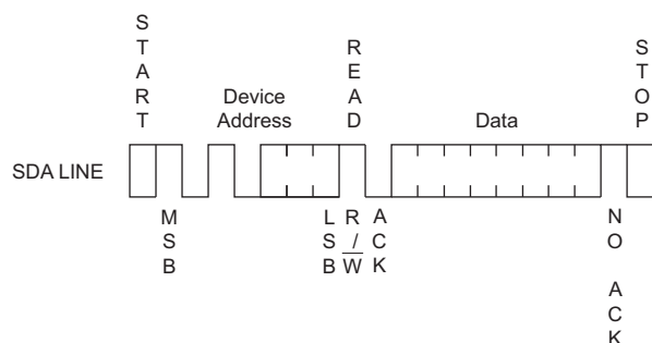
Figure 9-1. Current Address Read
