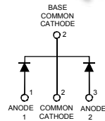
TO-220
