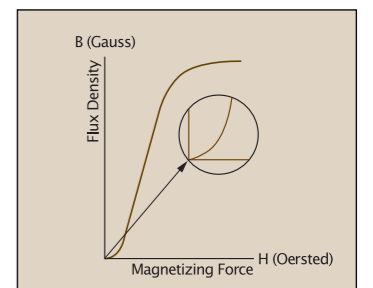
Figure 4. Initial Permeability
