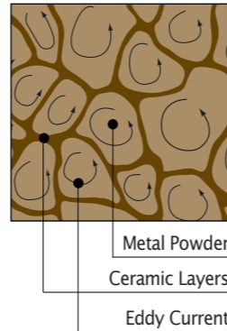
Figure 1. Eddy Current in Powder Cores
