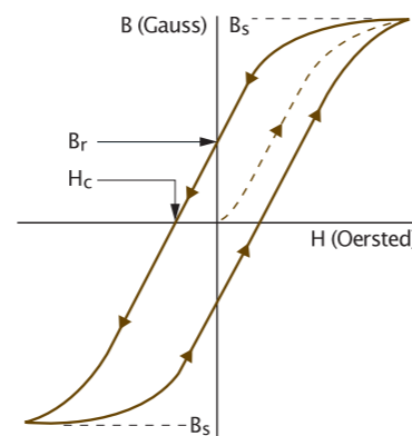
Figure 2. B-H Loop
