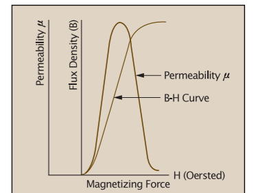
Figure 3. Variation of \mu along the Magnetization Curve
