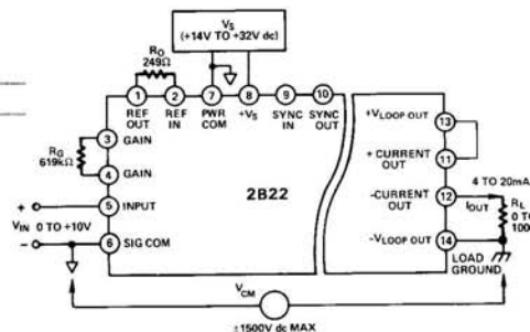
Figure 1. Basic Connections
