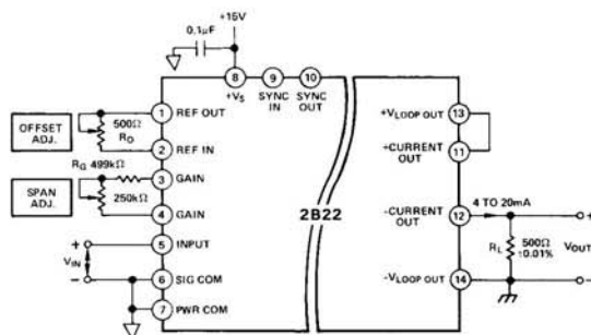
Figure 3. Optional Span and Offset Adjustment
