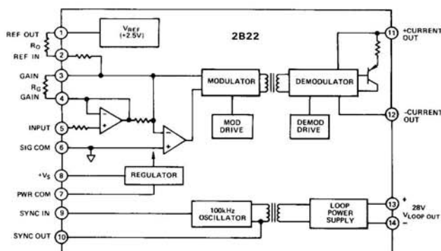
Figure 2. Block Diagram – 2B22
