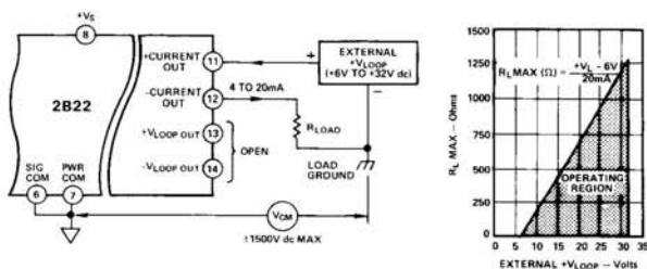
Figure 4. Optional External Loop Power Operation
