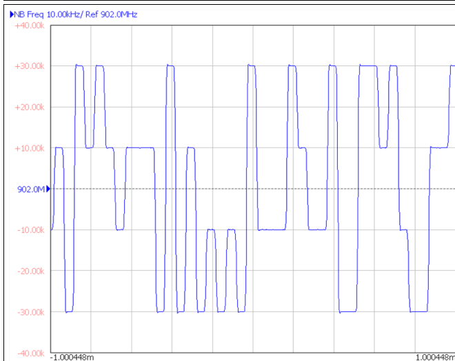
Figure 69. 4FSK Modulation
