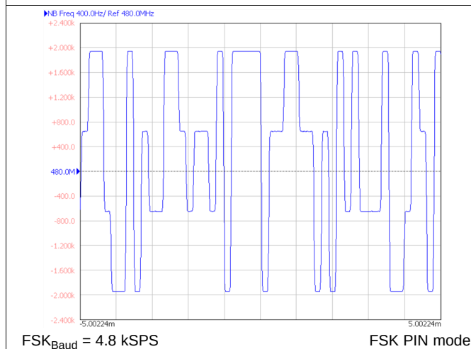
Figure 6. 4FSK Direct Digital Modulation
