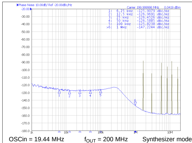
Figure 2. Typical Close Loop Phase Noise
