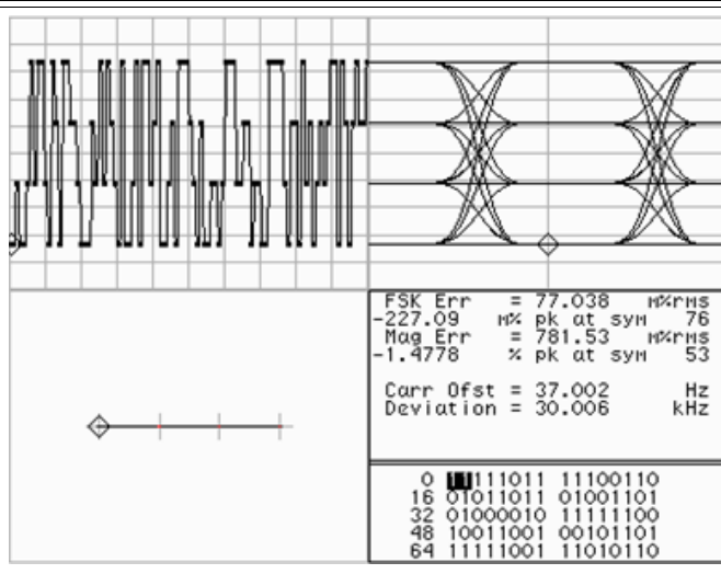
Figure 70. 4FSK Modulation Quality
