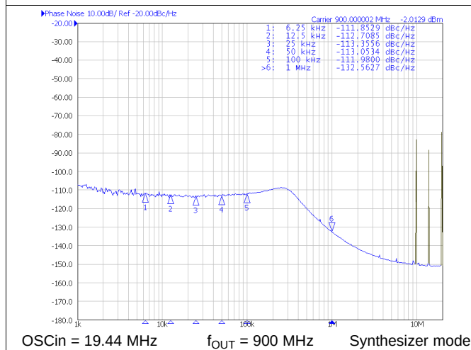
Figure 4. Typical Close Loop Phase Noise
