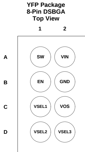
Pin Functions
