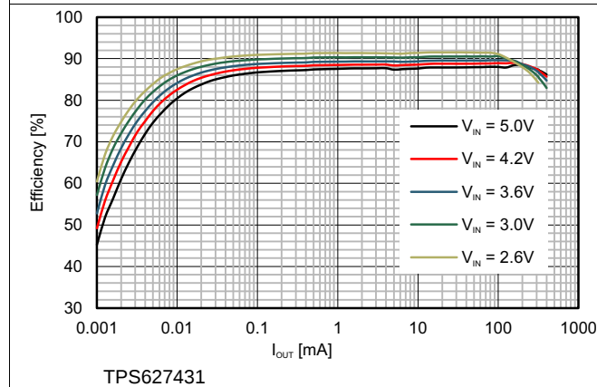
图 10. Efficiency vs Load Current; V_{OUT} = 1.9\text{ V}
