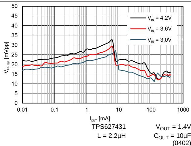
图 19. Typical Output Ripple Voltage V_{OUT} = 1.4\text{ V}
