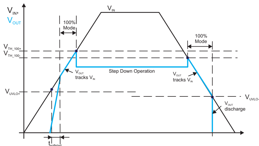
图 5. Automatic Transition into 100% Mode
