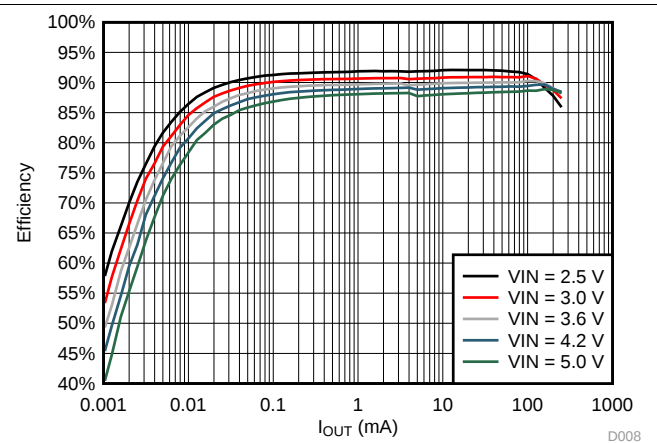
图 9. Efficiency vs Load Current; V_{OUT} = 2.1\text{ V}
