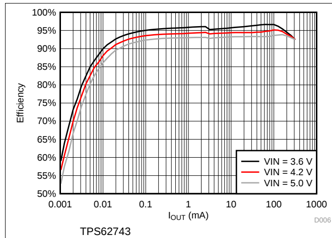
图 8. Efficiency vs Load Current, V_{OUT} = 3.3\text{ V}
