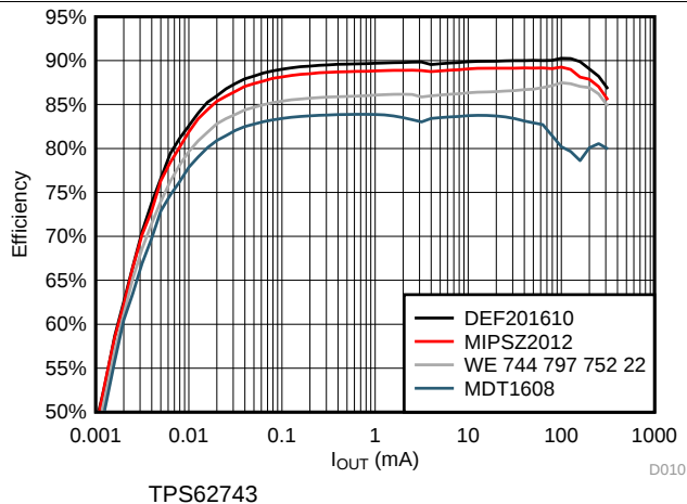
图 14. Efficiency vs Load Current; V_{OUT} = 1.8\text{ V}
