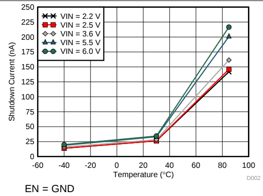
图 2. Shutdown Current I_{SD} vs Temperature
