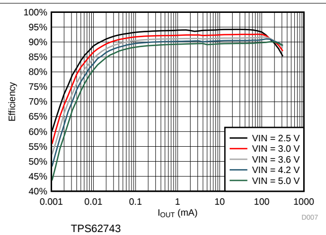
图 9. Efficiency vs Load Current; V_{OUT} = 2.1\text{ V}
