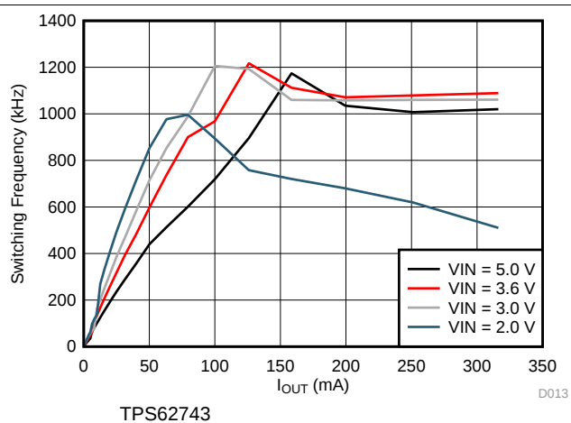
图 18. Switching Frequency vs Load Current V_{OUT} = 1.2\text{ V}
