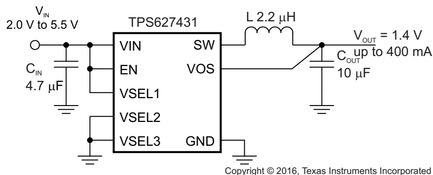
图 7. TPS627431 Typical Application Circuit
