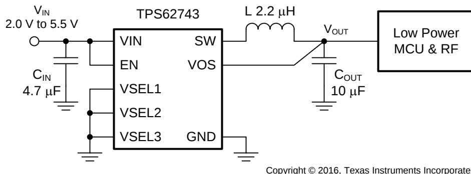
图 6. TPS62743 Typical Application Circuit
