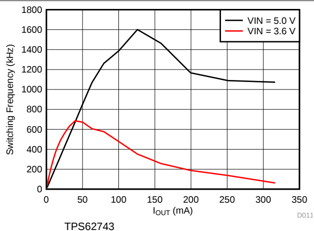
图 15. Switching Frequency vs Load Current V_{OUT} = 3.3\text{ V}
