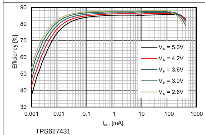
图 12. Efficiency vs Load Current; V_{OUT} = 1.4\text{ V}
