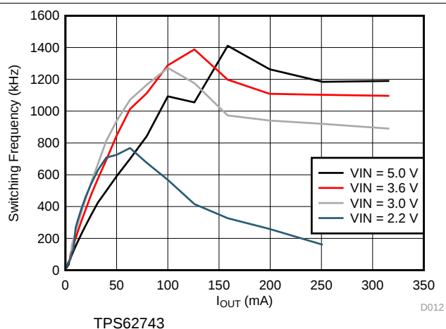
图 16. Switching Frequency vs Load Current V_{OUT} = 1.8\text{ V}
