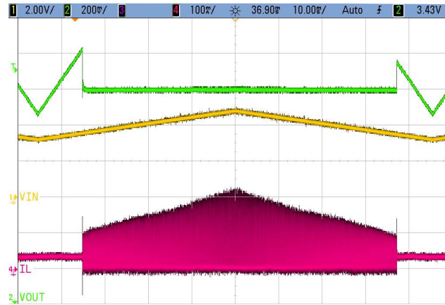
图 26. 100% Mode Entry and Leave Operation I_{OUT} = 30 \text{ mA}
