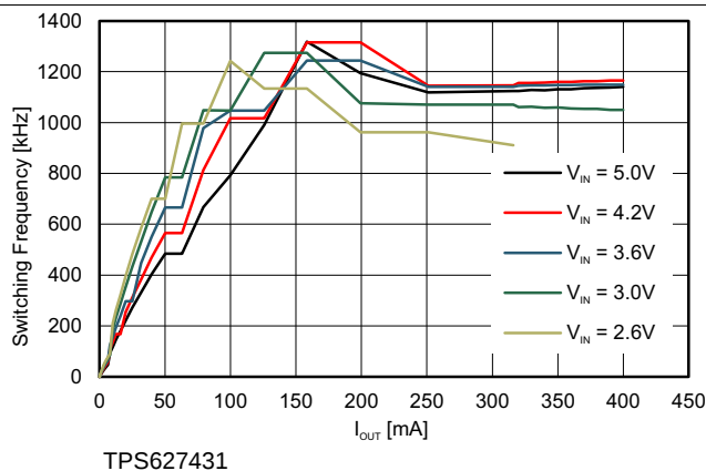
图 17. Switching Frequency vs Load Current V_{OUT} = 1.4\text{ V}
