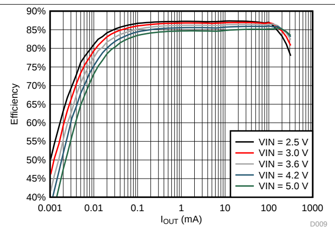
图 11. Efficiency vs Load Current; V_{OUT} = 1.8\text{ V}
