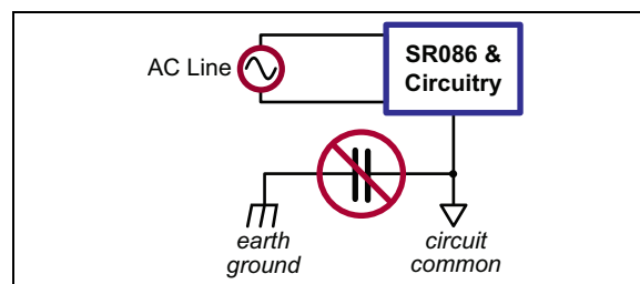
FIGURE 3-4: EMI Capacitor.
