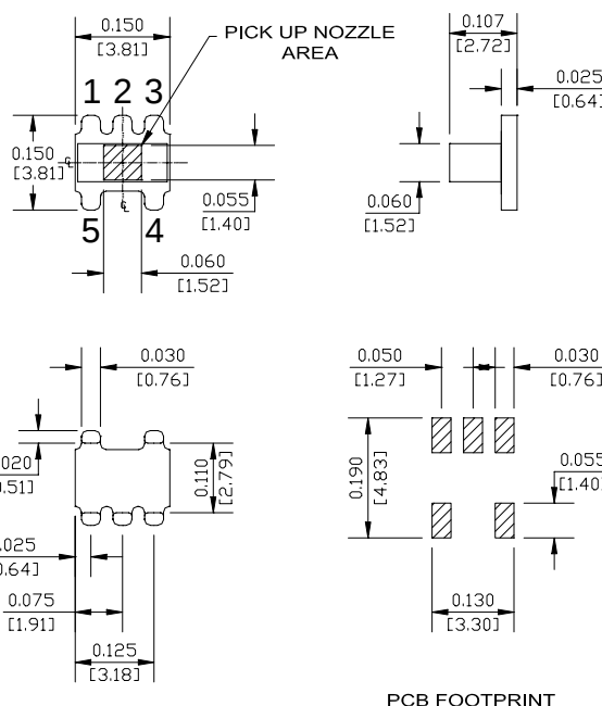
PCB FOOTPRINT
