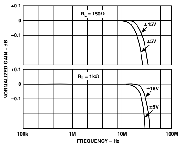
Figure 1. Fine-Scale Gain (Normalized) vs. Frequency for Various Supply Voltages, R F = 750 Ω, Gain = +2
