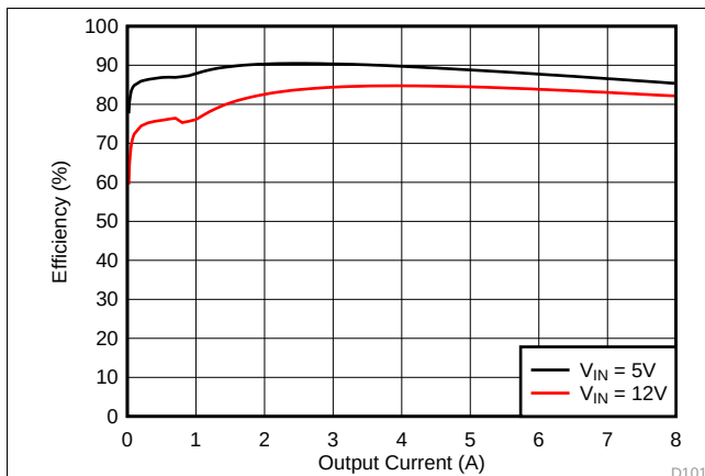
Figure 23. Efficiency
