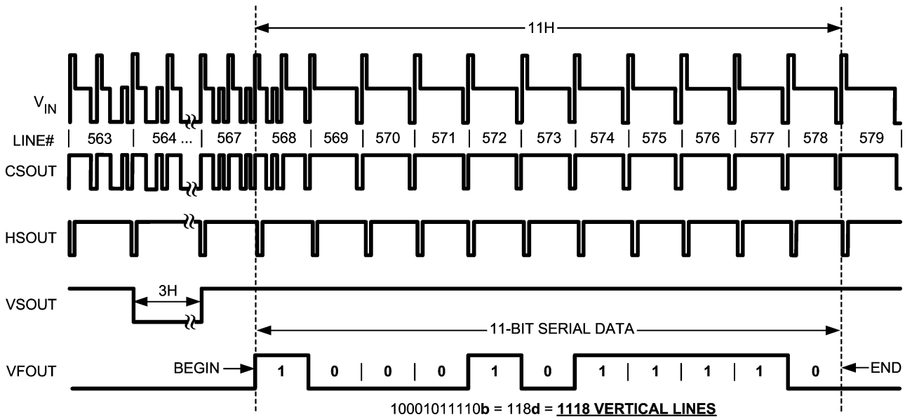
FIGURE 12. Video Format Output for Interlaced Format, 1080i Field 2
