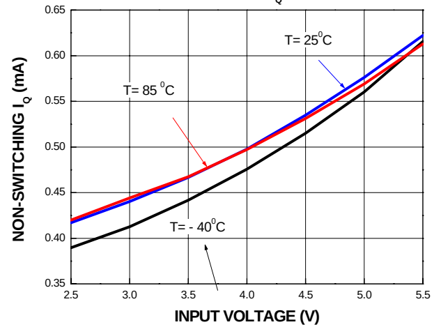
1.25MHz Non-switching I_Q vs. Input Voltage
