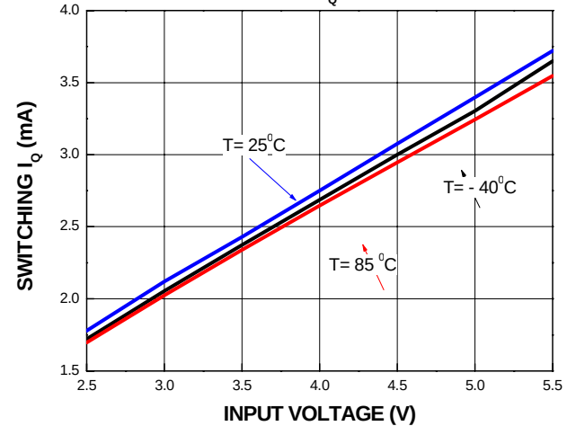
1.25MHz Switching I_Q vs. Input Voltage
