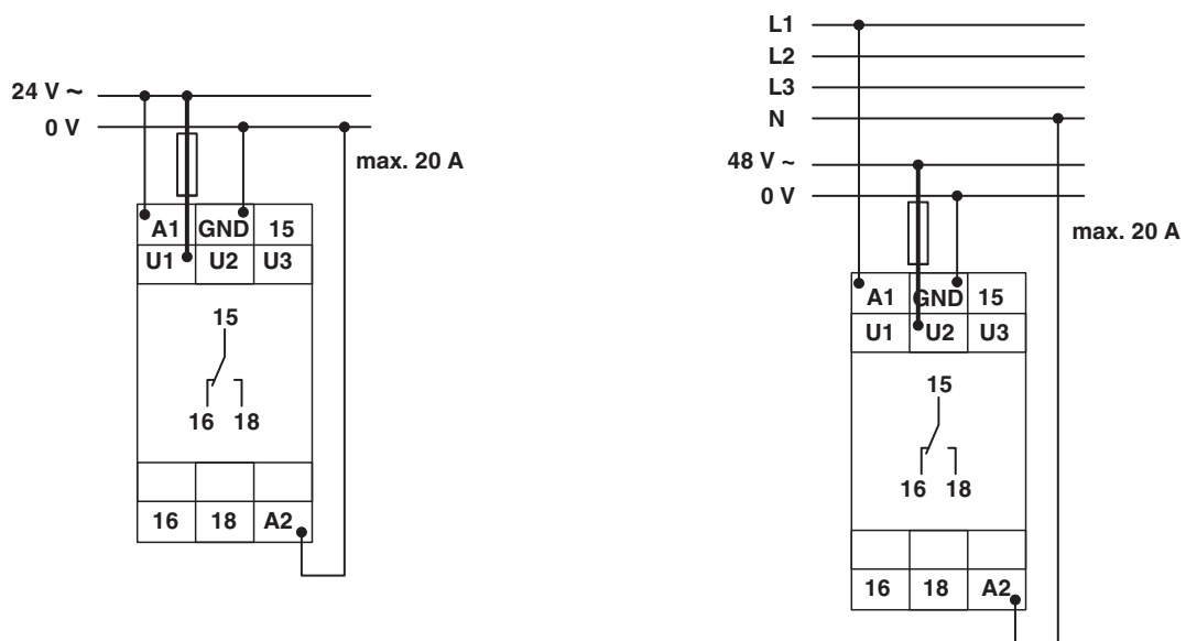
30 V (U1) measuring range with 24 V AC power module
