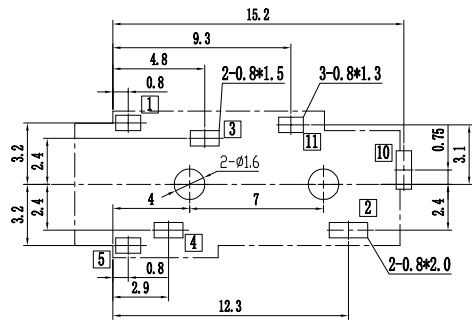
PCB LAYOUT (TOP)
