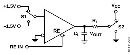
Figure 28. Receiver Enable/Disable
