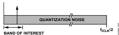
Figure 82. \Sigma - \Delta ADC Operation, Reduction of Noise Energy Contained in the Band of Interest (Linear Scale X-Axis)
