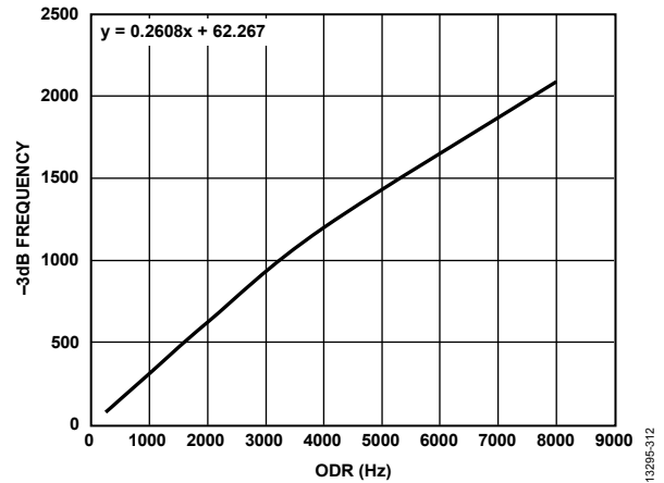
Figure 113. -3 dB Correction Factor, LP Mode
