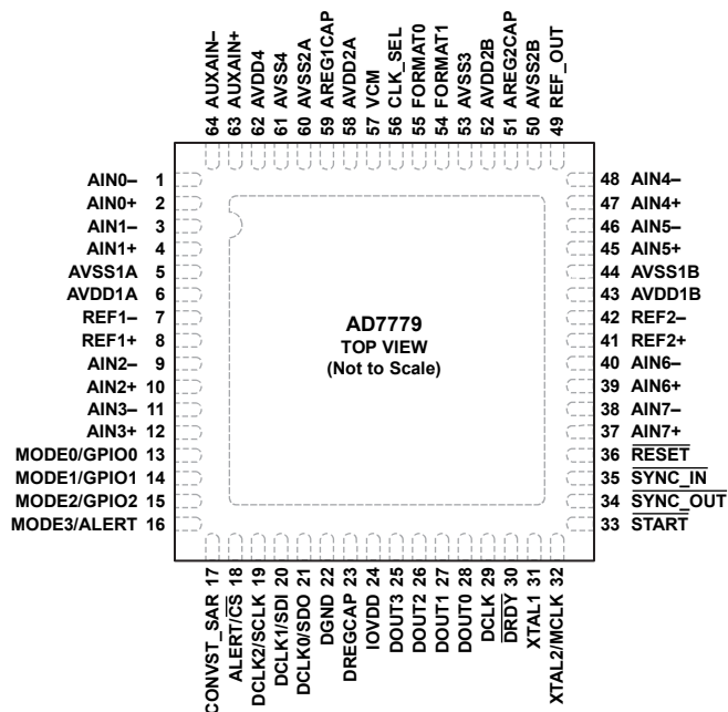
Figure 7. Pin Configuration
