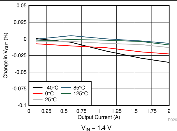
Figure 7-26. Load Regulation
