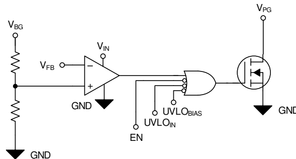
Figure 8-4. Simplified PG Circuit
