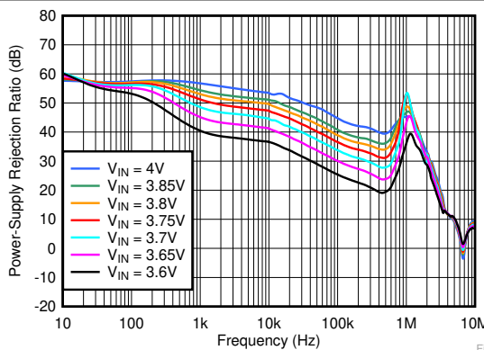
Figure 7-4. PSRR vs Frequency and V_{IN}
