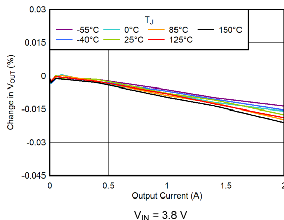
Figure 7-52. Load Regulation (3.3-V Output)
