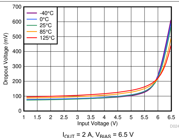
Figure 7-21. Dropout Voltage vs Input Voltage With BIAS
