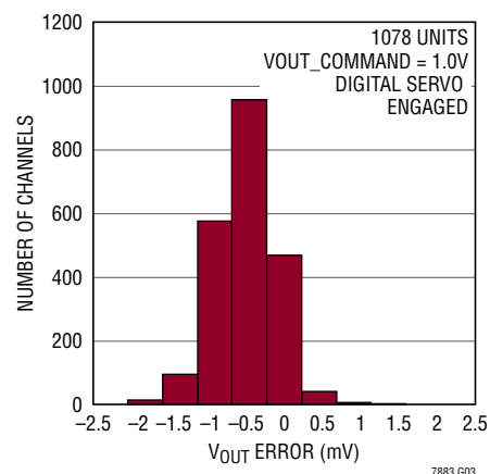
Typical LTC7883 Output Voltage Distribution at 105°C
