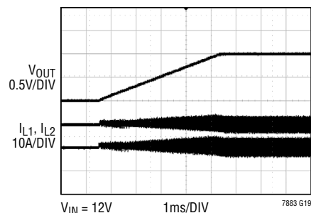
Soft-Start Ramp
