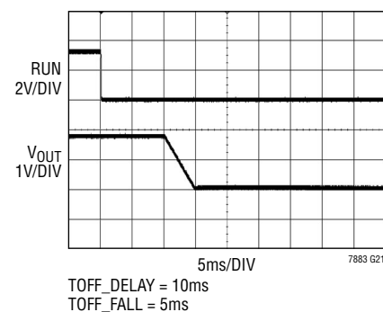
Soft-Off Ramp
