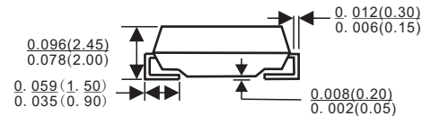
Dimensions in inches(millimeters)
