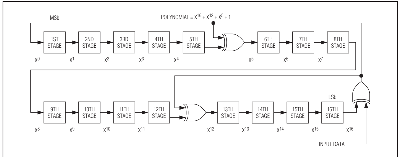
Figure 32. CRC-16-CCITT Generator
