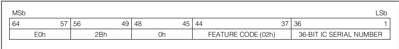
Figure 3. 64-Bit UID
