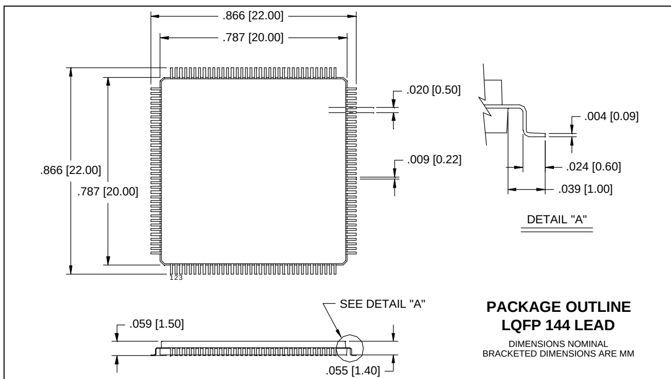
Figure 30: Physical Dimensions
