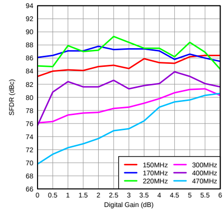
图 35. SFDR vs Gain and Input Frequency
