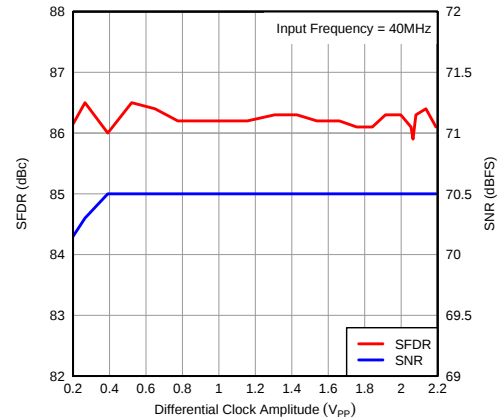
图 85. Performance vs Input Clock Amplitude
