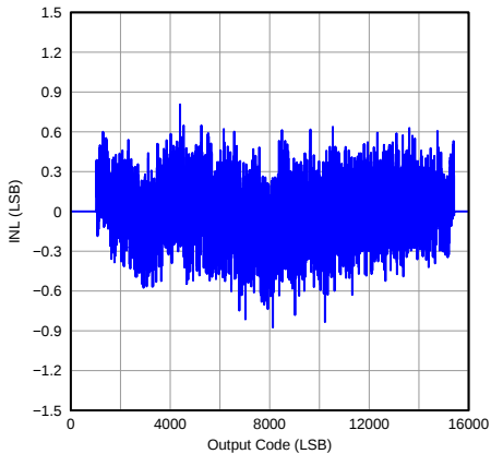
图 68. Integrated Nonlinearity
