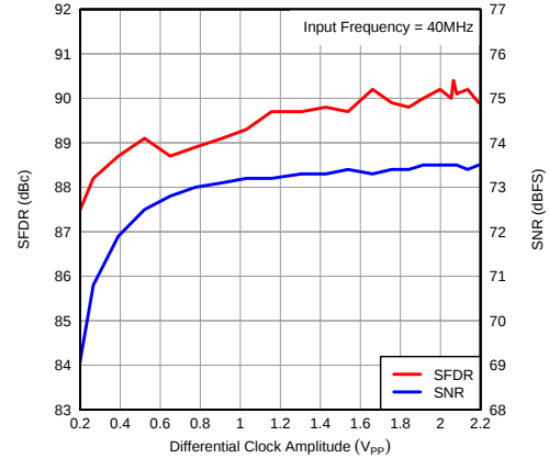
图 65. Performance vs Input Clock Amplitude
