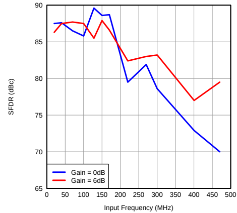
图 91. SFDR vs Input Frequency
