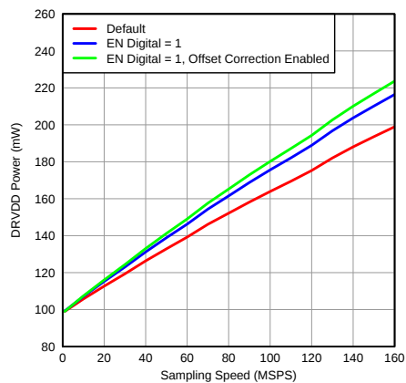
图 128. Digital Power in Various Modes (LVDS)
