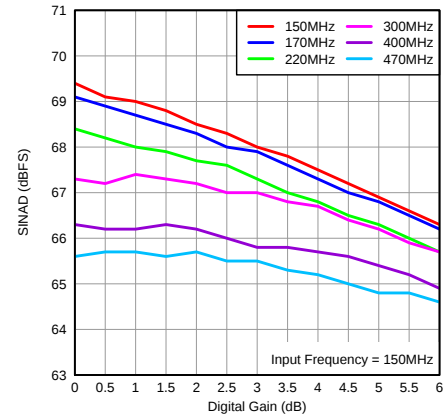
图 113. SINAD vs Gain and Input Frequency
