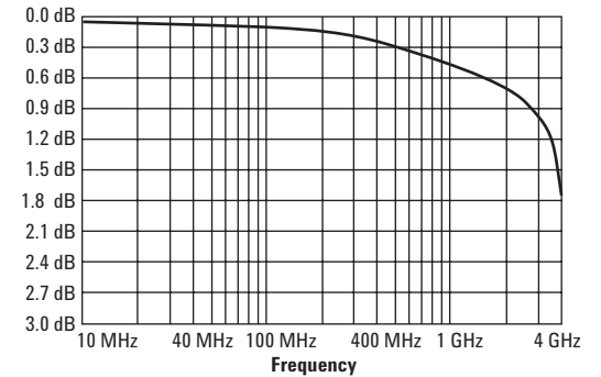
34941A typical initial insertion loss
