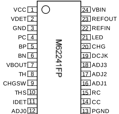
PIN configuration (Top view)
