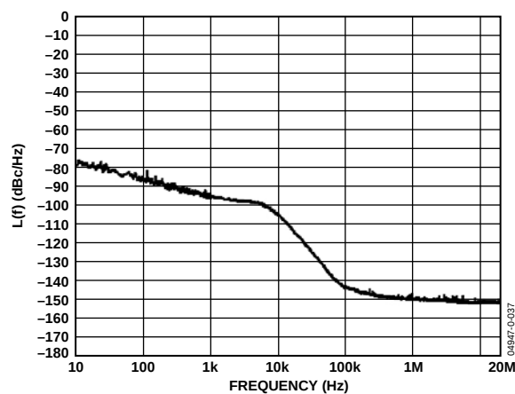
Figure 30. Total System Phase Noise for 210 MHz Converter Clock
