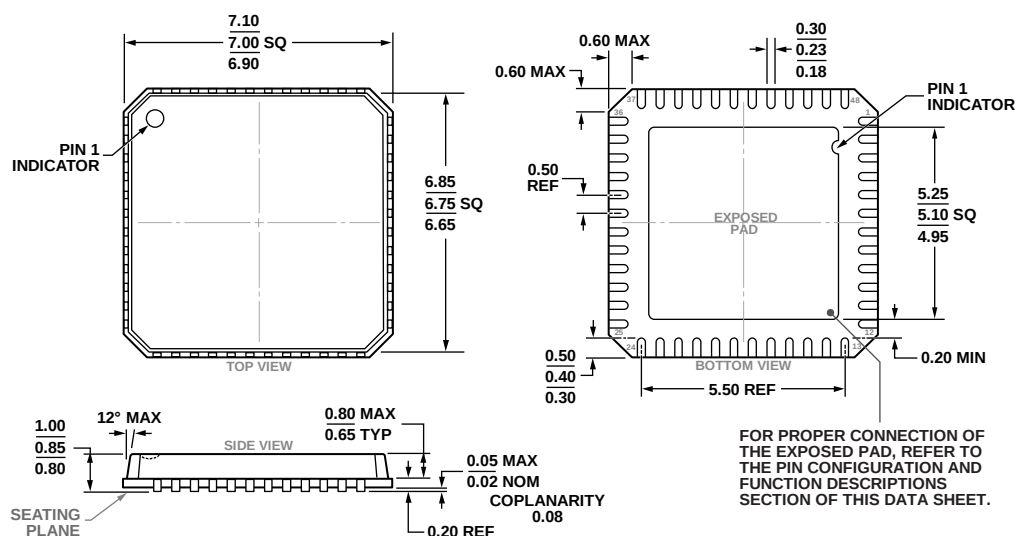
Figure 45. 48-Lead Lead Frame Chip Scale Package [LFCSP] 7 mm × 7 mm Body and 0.85 mm Package Height (CP-48-1)
