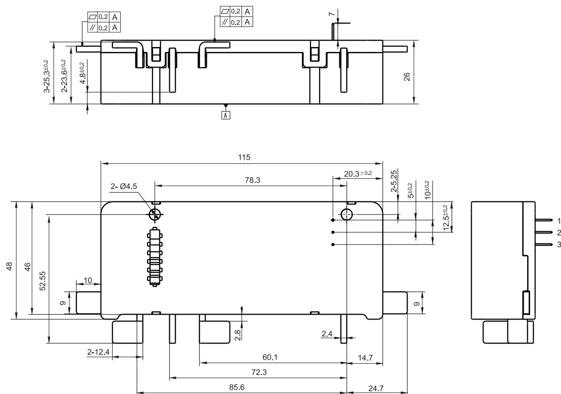
Outline Dimensions
