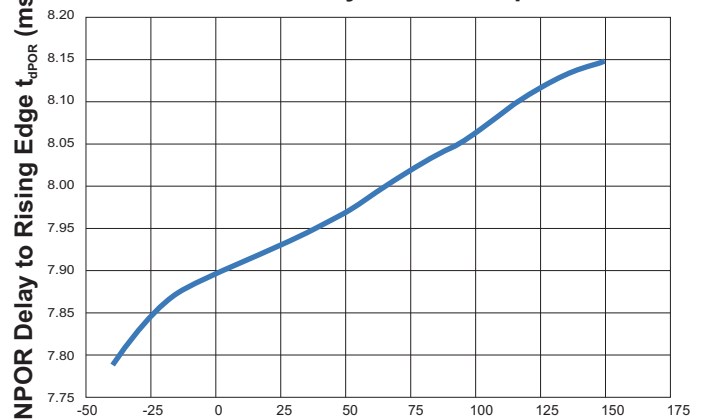
NPOR Time Delay to Rising Edge versus Temperature
