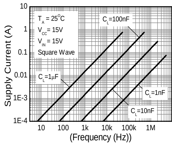
Supply Current
