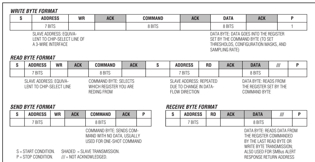
Figure 2. SMBus Protocols
